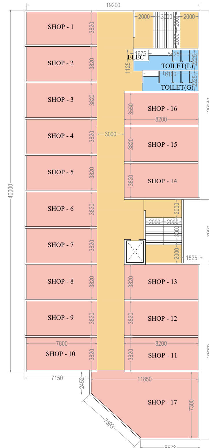
FIRST & SECOND FLOOR PLAN (TYPICAL)
